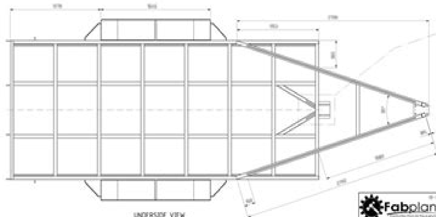
UNDERSIDE VIEW
